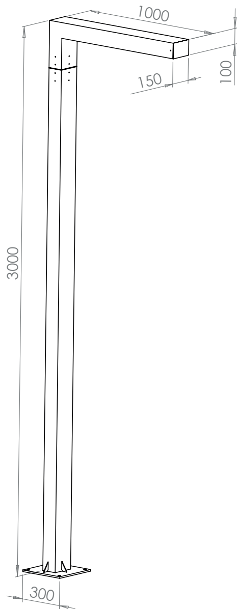
GTM-FN 6-90 3000
