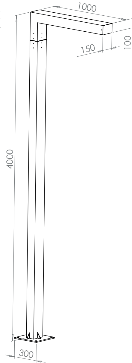
GTM-FN 6-90 4000
