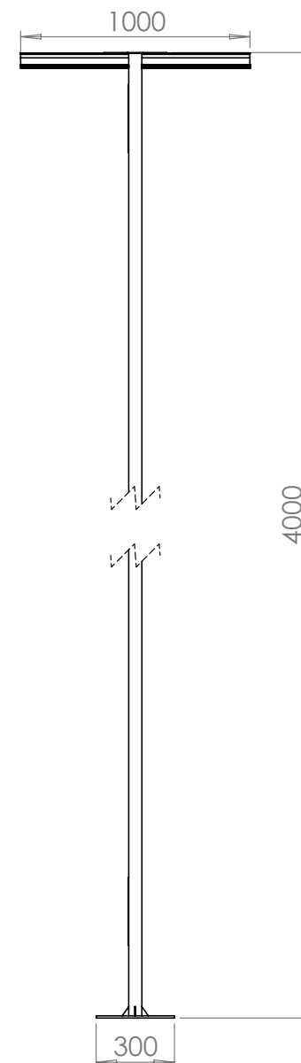
GAL-FN 2-90 4000
