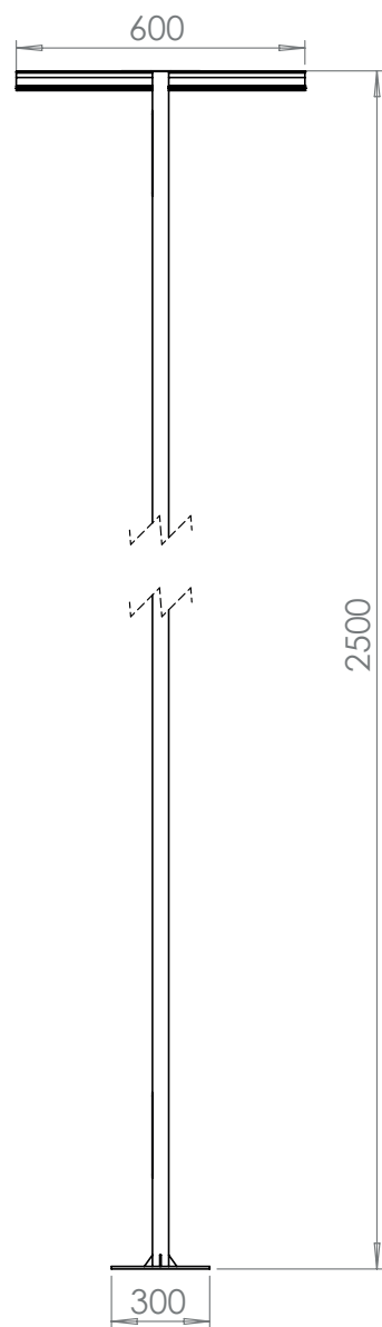
GAL-FN 2-90 2500
